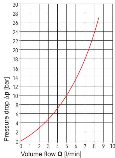
\Delta p -Q nominal line for kinematic viscosity of 53 \times 10^{-6} \text{ m}^2/\text{s} (HLP 22 at 20° C)
