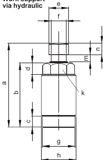
Work support via hydraulic
