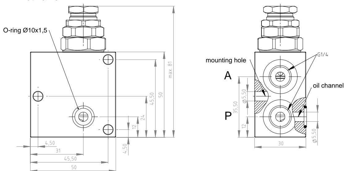
Inlet valve
