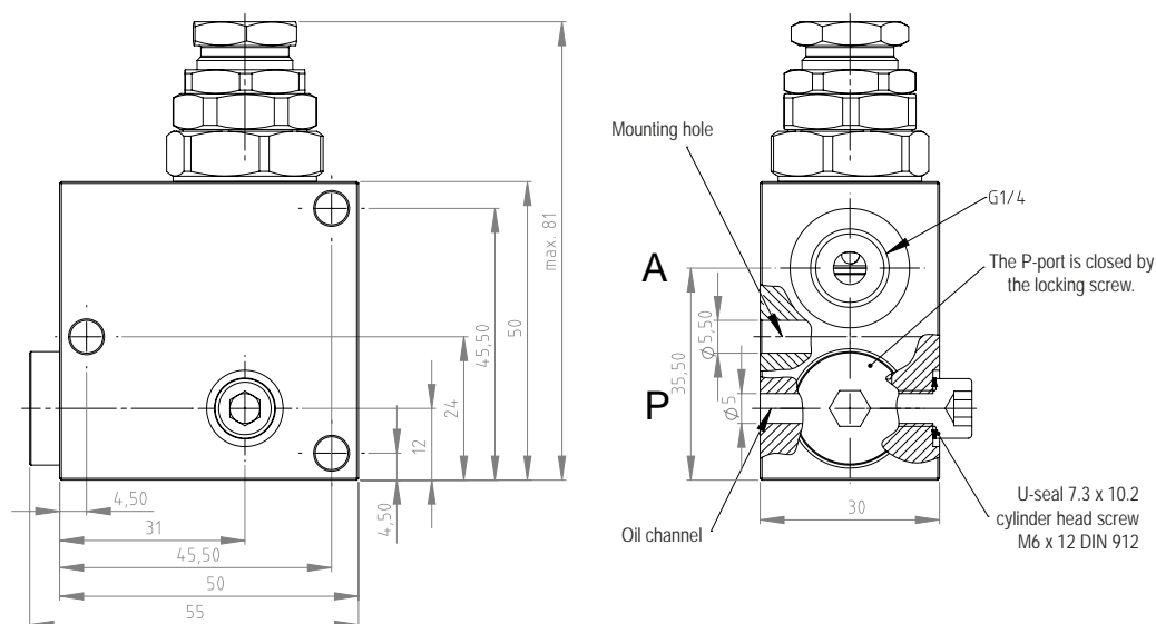
Series valve
